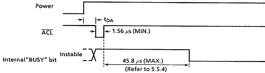
Fig.5.17 \overline{ACL} pulse width
