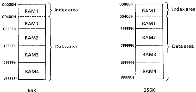
Fig.5.12 Memory map in level index mode
