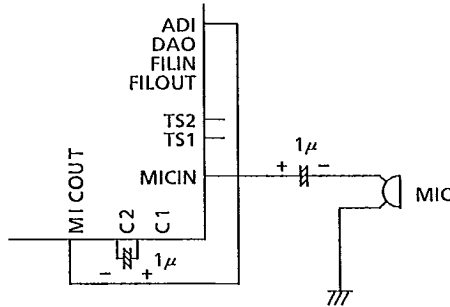
Fig.5.24 Connection of MIC
