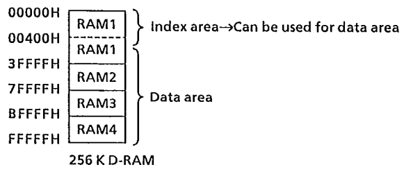
Fig.5.7 Memory map at direct mode
