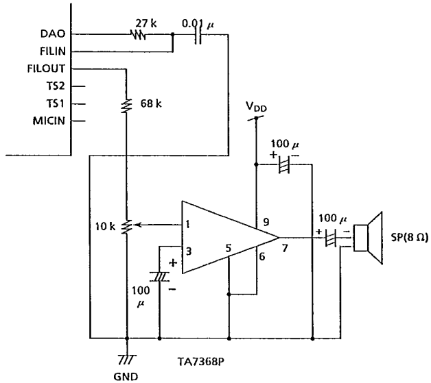
Fig.5.26 Connection of audio amp.
