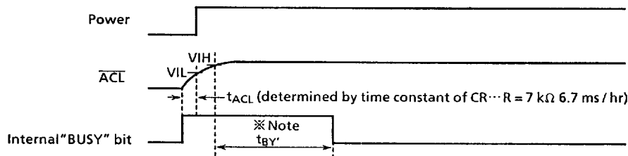
Fig.5.19 \overline{ACL} input at power on reset
