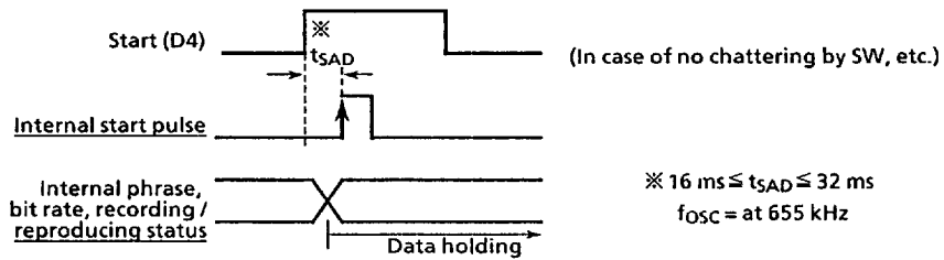
Fig.5.3 Start input and internal status
