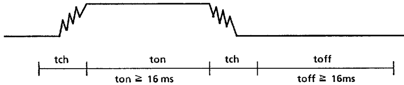
Fig.5.5 Chattering preventing circuit
