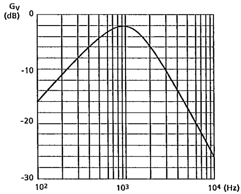
Fig.5.27 Frequency characteristics of band pass filter
