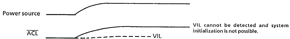
Fig.5.20 In case power rise is gentle
