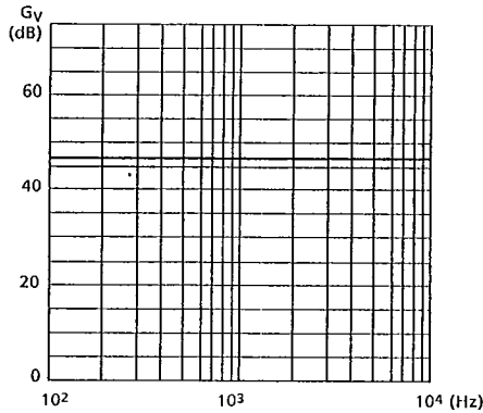
Fig.5.25 Frequency characteristics of MIC. AMP.
