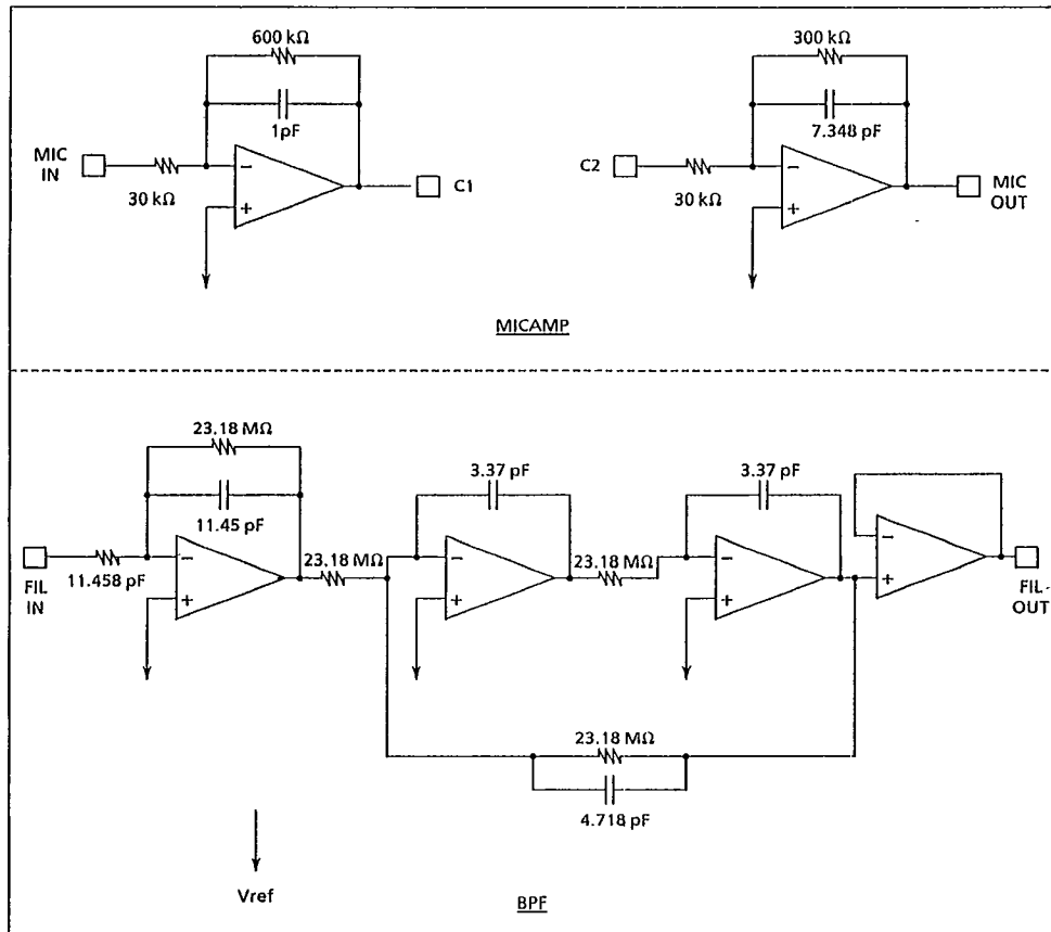
Fig.5.28 Equivalent circuits of analog circuits
