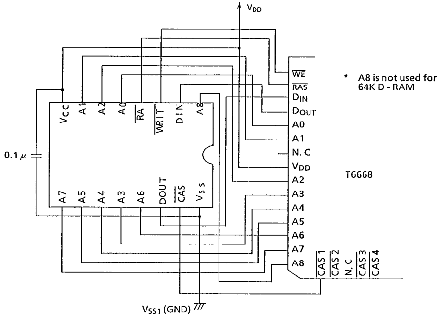
Fig.5.23 Connection with D - RAM
