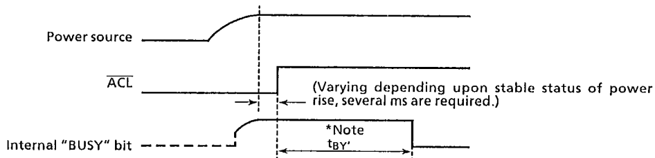
Fig.5.21 System initialization by CPU control
