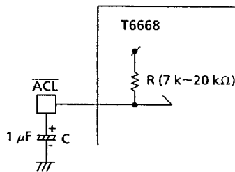
Fig.5.18 Circuit for power on reset
