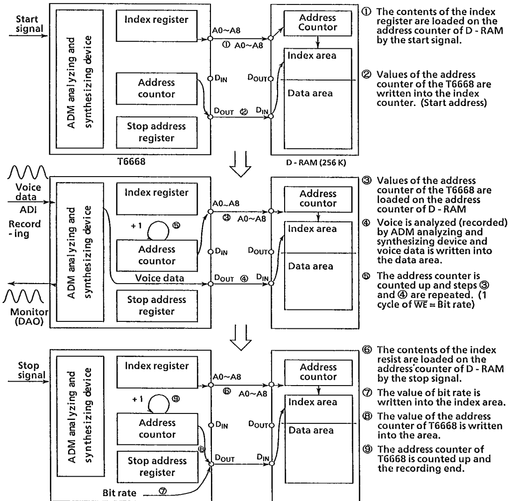
Fig.5.15 Access to memory in recording
