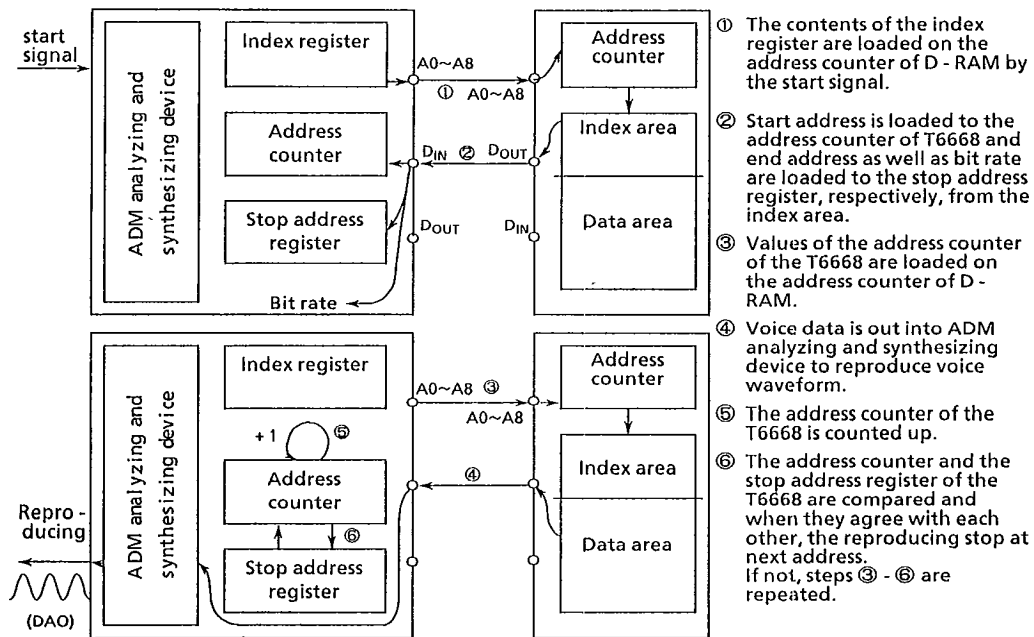
Fig.5.16 Access to memory in reproducing
